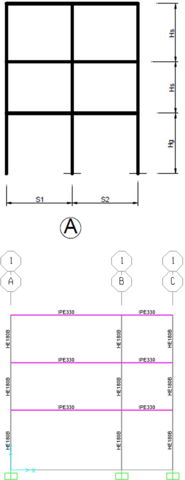
Figure 1. Structural model of the steel building.
