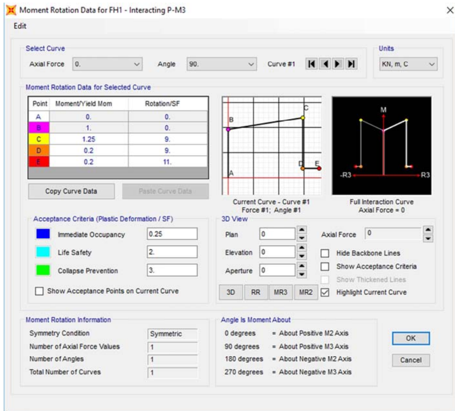
Figure 2. Properties for push over analysis
