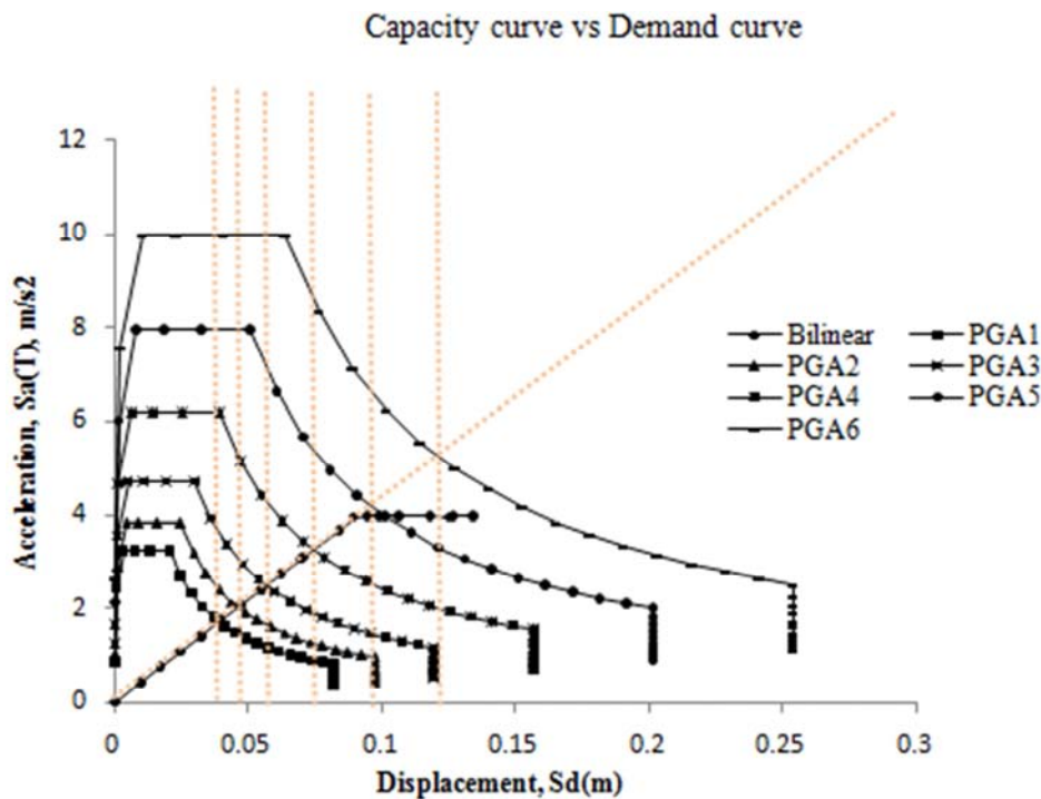
Figure 9. Capacity-demand curve of initial structure.
