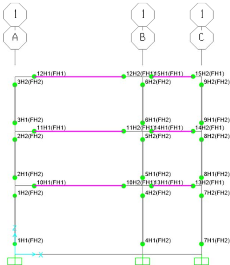
Figure 3. Hinge assignment to members.
